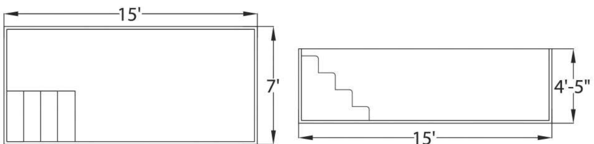
RECTANGULAR SWIMMING POOL - (15'X7'X4.5") MODEL - L & R
