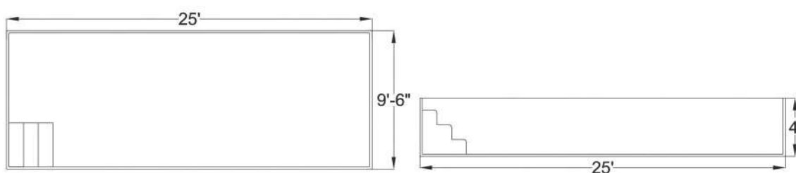
RECTANGULAR SWIMMING POOL - (25'X9.6'X4') MODEL - W3
